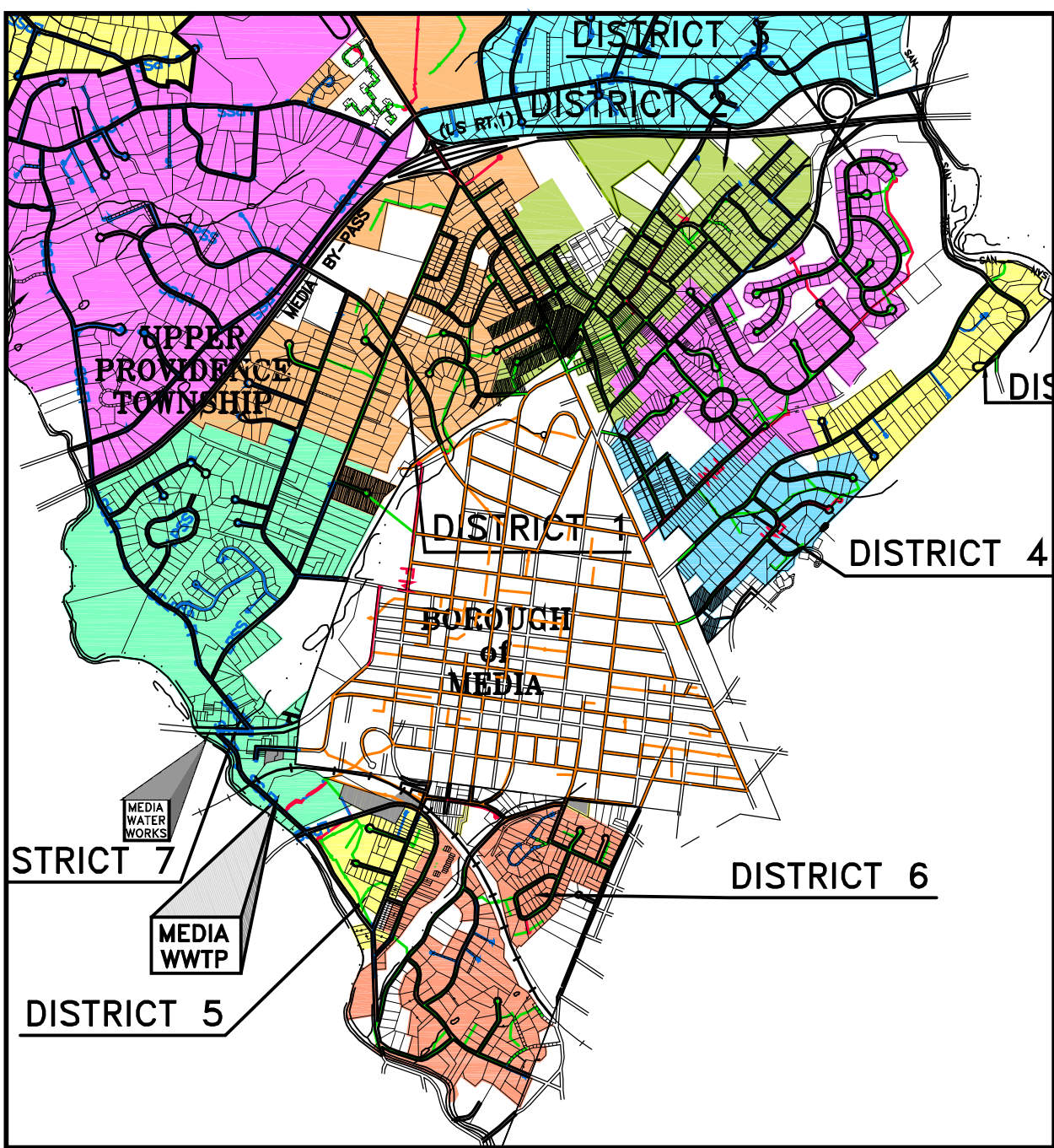
SANITARY SEWER DISTRICT LOCATION MAP SCALE: 1" = 2,000'
